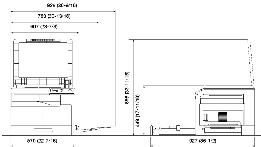
bizhub 164 + MB-503
